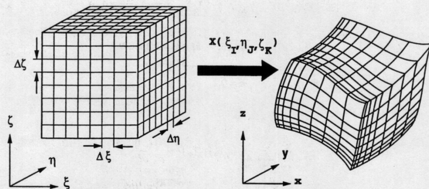
FIGURE 3.2 Grids in computational and physical domains.
